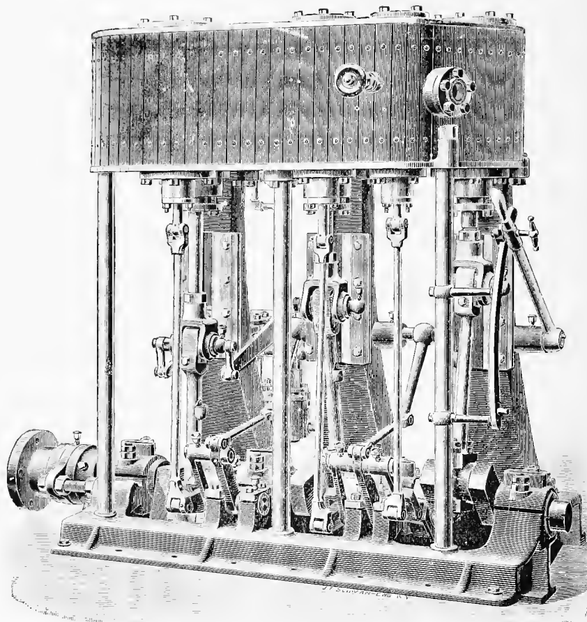
SULLIVAN'S TRIPLE-EXPANSION YACHT ENGINE.
